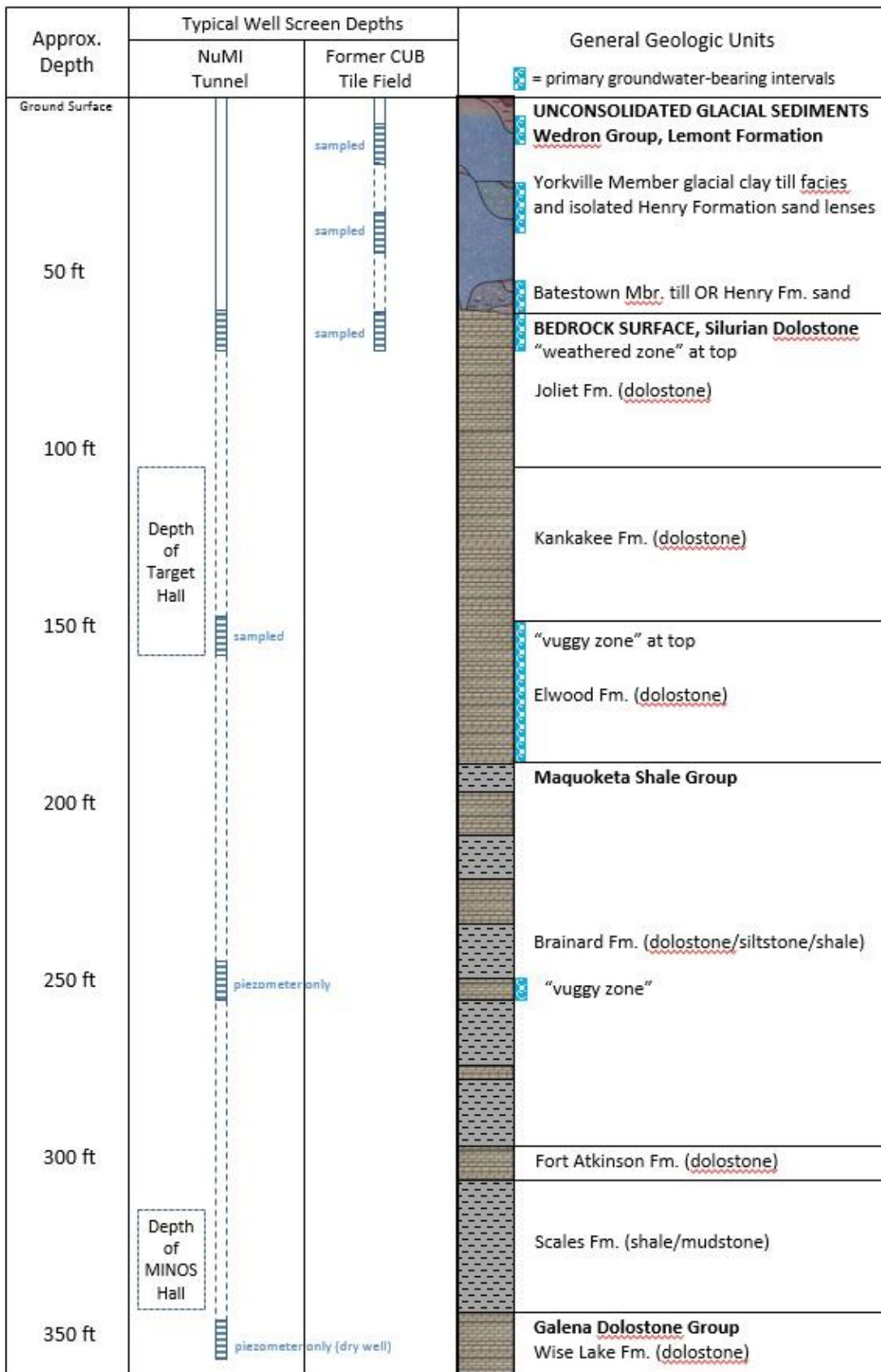
Figure 6.4-1. General Fermilab geologic section (based on the NuMI tunnel), with groundwater monitoring
