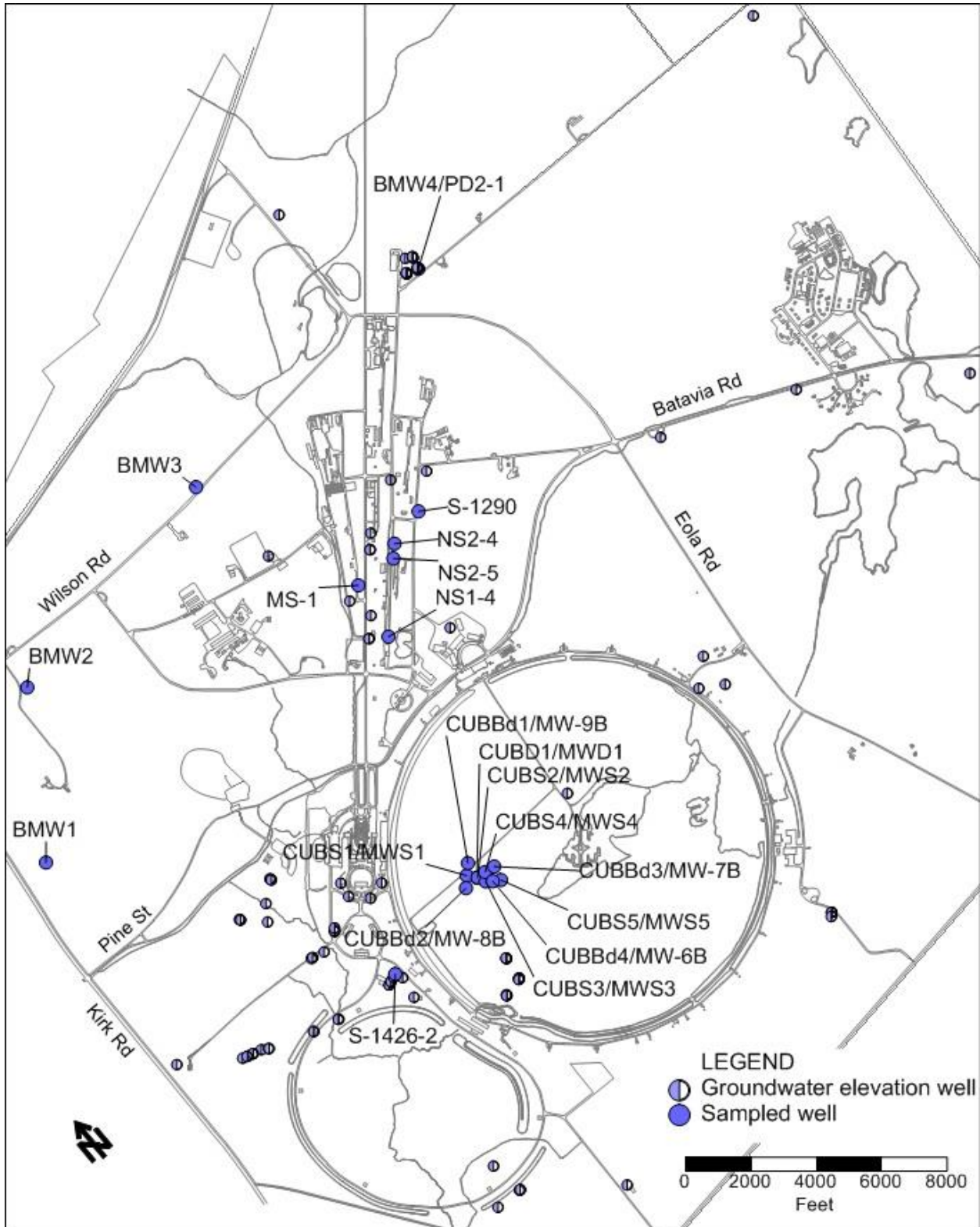
Figure 6.4-2. Groundwater monitoring well locations in 2018. Sampled wells represented by labeled, filled circles. Wells used only for groundwater elevations represented by half-open circles. (Original DUSAF projection)
